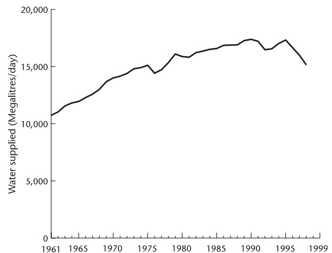
Figure 1. Water consumption in the U.K. (1961–2000).
