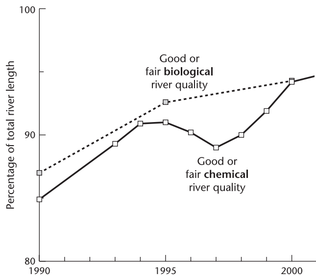
Figure 6. Biological and chemical river quality (1990–2000).
